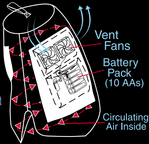
TT45712AF Hood with Fresh Air System (Rear View Diagram)
